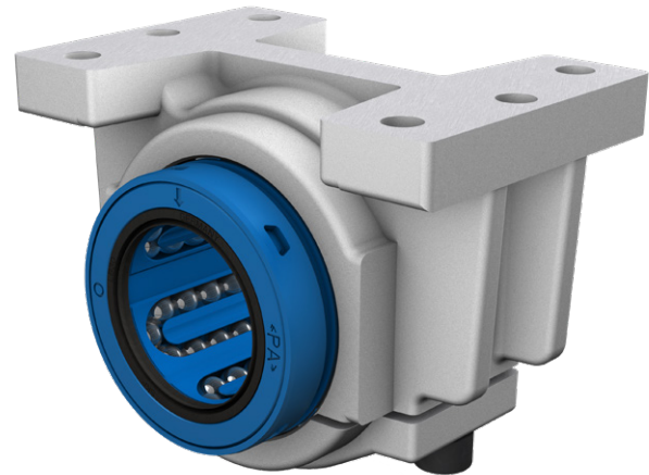
Pictured is LUCE 30 D-2LS 2)
