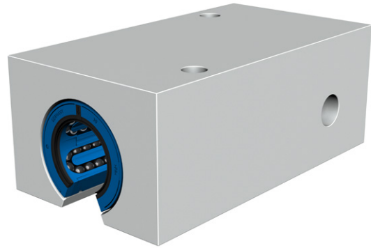
Pictured is LTCF 30 D-2LS 2)
