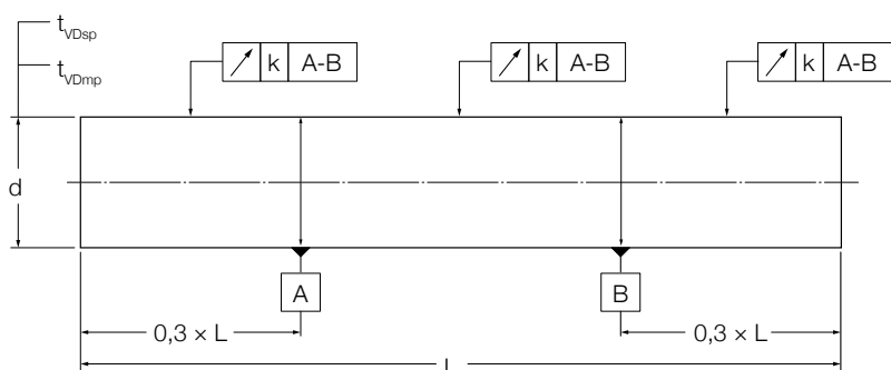
Definition of shaft tolerances is according to ISO 13012-1
