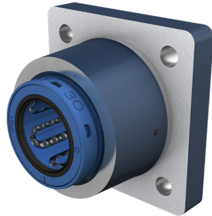
Pictured is LVCR 30 D-2LS 2)
