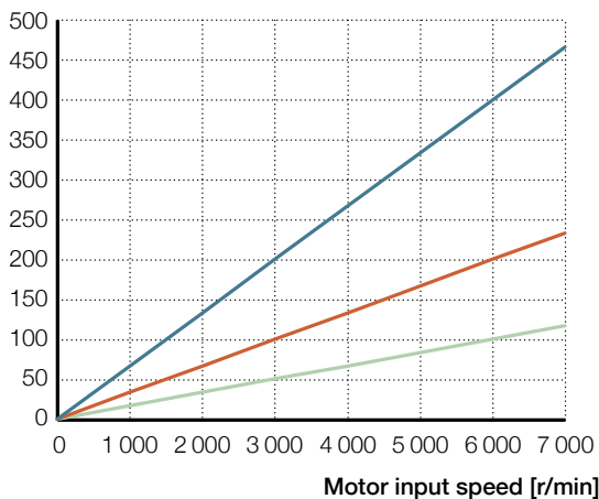
Pillar output speed [mm/s]
